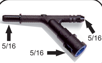
106-150-040 Conector 45° Pop Top 5/16 x 5/16 x5/16
