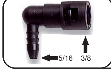
106-150-033 Conector 90° Pop Top 3/8x 5/16
