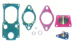
107-200-052 Kit p/ Carb. Solex F-1000 / Veraneio/ Rural Simples/ Jeep 40 DEIS - Gas/Alc
